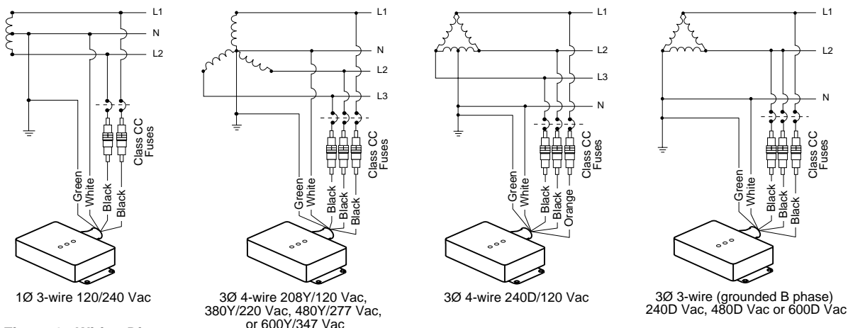
Figure 1: Wiring Diagrams
