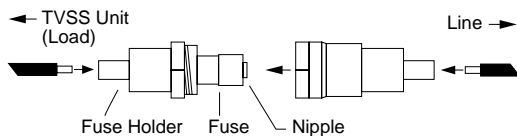
Figure 3: Connecting TVSS Unit to Fuse Holder and Circuit Breaker
