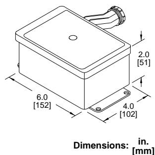
Figure 5: Dimensions
