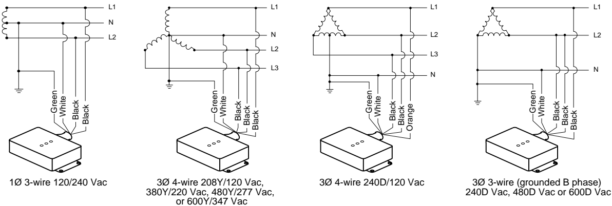
Figure 1: Wiring Diagrams
