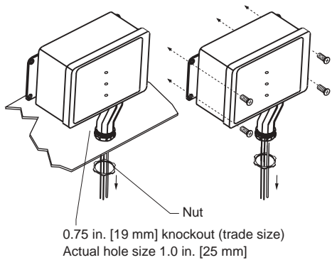
Figure 2: Mounting Unit
