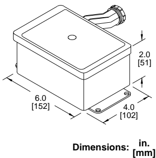
Figure 4: Dimensions
