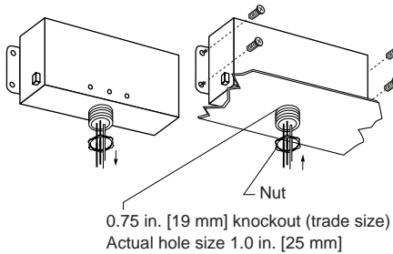
Figure 2: Mounting Unit
