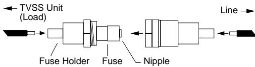
Figure 3: Connecting TVSS Unit to Fuse Holder and Circuit Breaker
