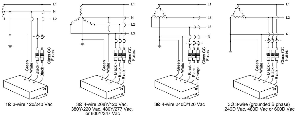
Figure 1: Wiring Diagrams
