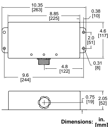
Figure 5: Dimensions
