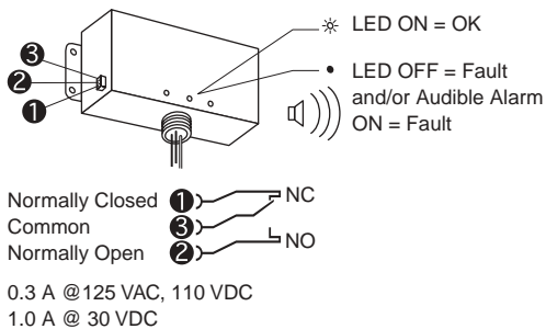
Figure 4: Remote Monitoring and Diagnostic Operation
